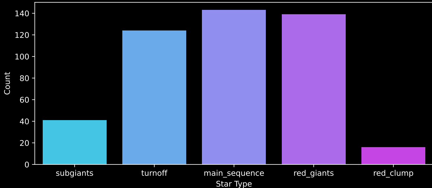
GALAH DR4 Field: [6787] Count plot of Star Type
