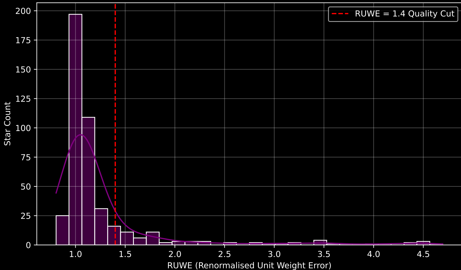
GALAH DR4 Field [6787] RUWE Distribution (n= 439)
