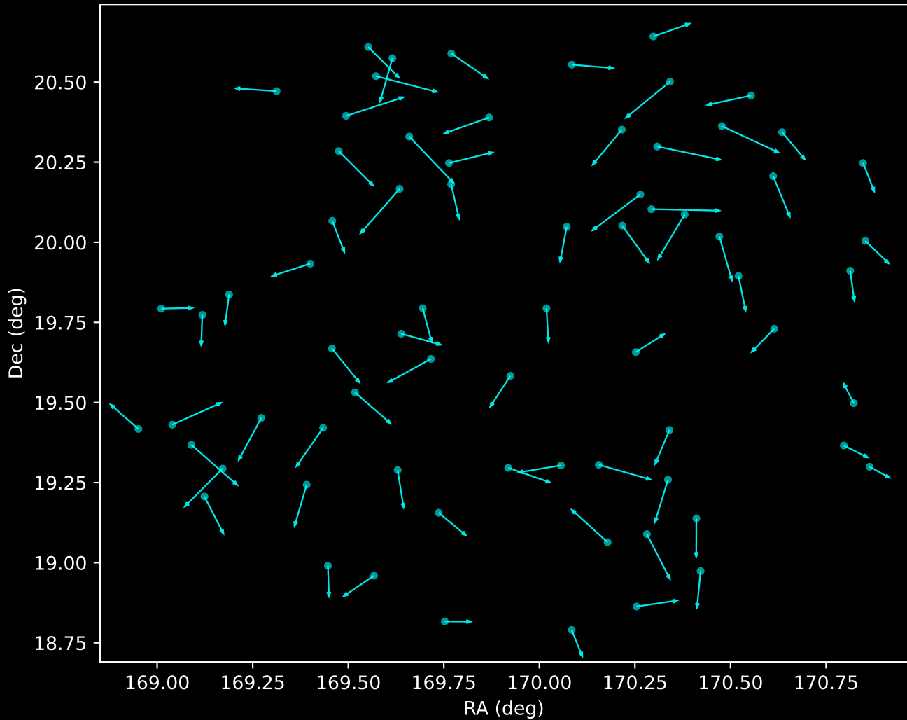
GALAH DR4 Noise Stream Proper Motion Vectors (n=72)
