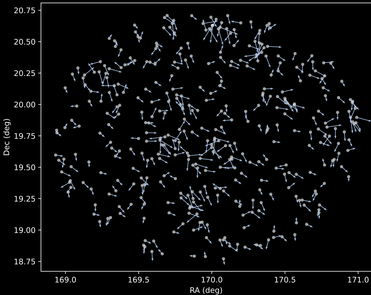
GALAH DR4 Cluster 1 Proper Motion Vectors (n=385)
