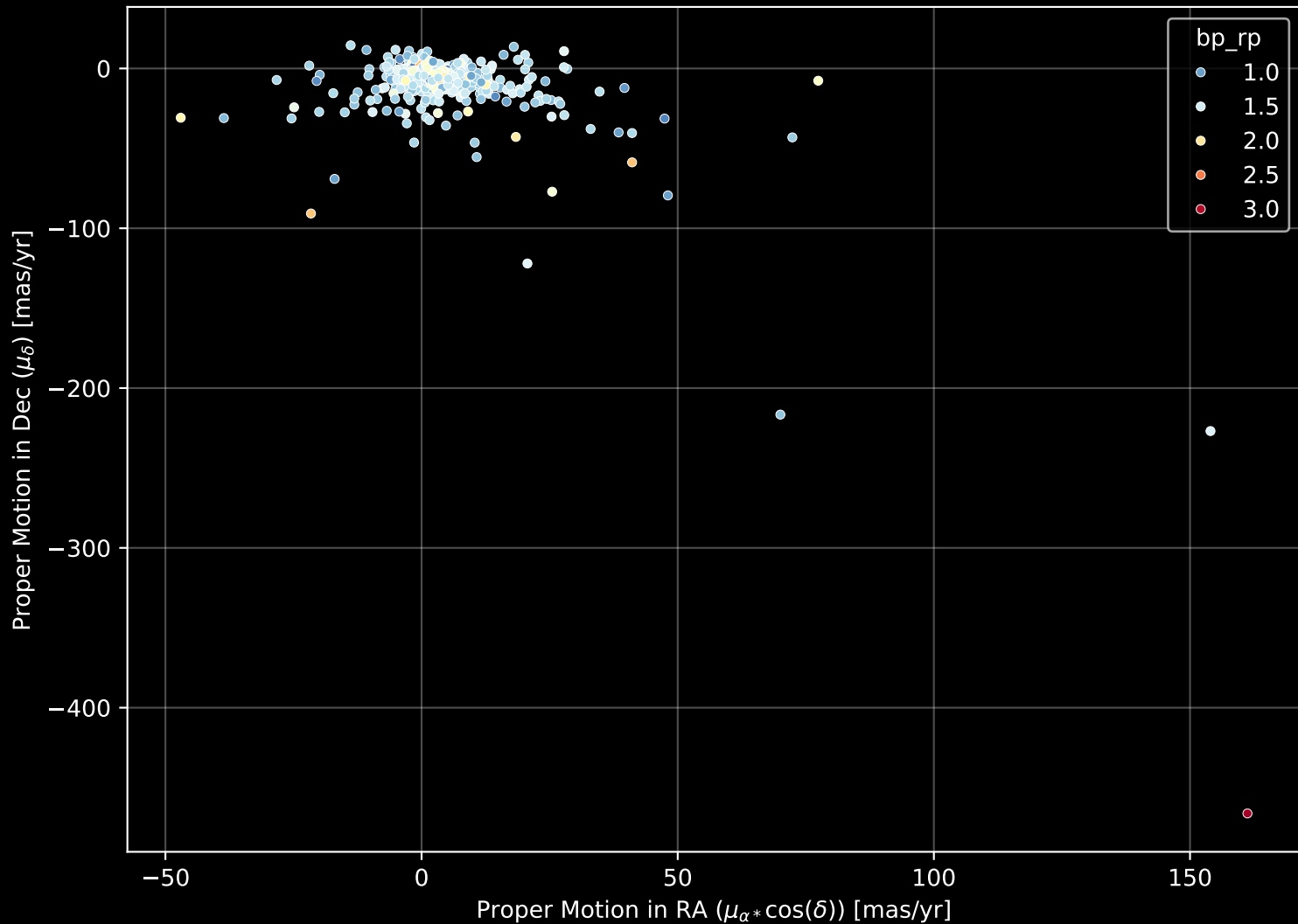
GALAH DR4 Field: [6787] Proper Motion Diagram (n= 463)
